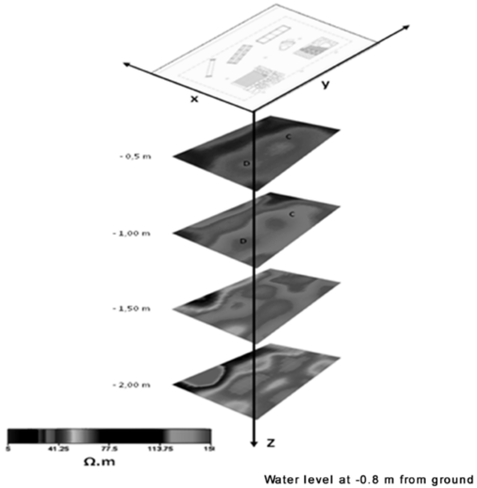
FIG. 6. 3D ELECTRICAL RESISTIVITY IMAGE AT DIFFERENT DEPTHS (DEPTH SLICES).
