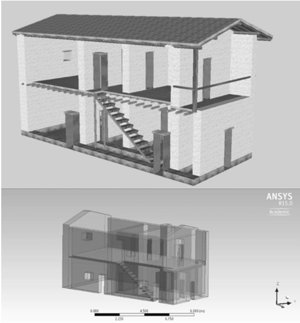
FIG. 5. TOP: VISUALIZATION OF THE 3D MODEL (WITH SOME WALLS REMOVED TO SHOW INTERIOR); BOTTOM: ANSYS MODEL WITH ROOF REMOVED.
