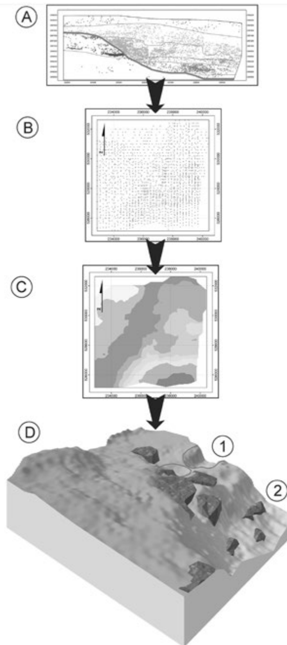
FIG. 7. 3D RECONSTRUCTION OF AN EROSIONAL PALAEOSURFACE OF THE COVA GRAN DE SANTA LINYA SITE (SOUTHERN PYRENEES, NE SPAIN) CREATED FROM THE CROSS SECTIONS. A: STRATIGRAPHIC CONTACTS ARE MODELLED AS LINES IN THE CROSS SECTIONS; B: LINES ARE AUTOMATICALLY CONVERTED INTO A XYZ POINT GRID; C, D: 3D SURFACES ARE OBTAINED BY INTERPOLATION METHODS. 1: NEOLITHIC PITS AND HEARTHS EXCAVATED IN THE PLEISTOCENE FLOOR; 2: EROSIONAL VOID.
