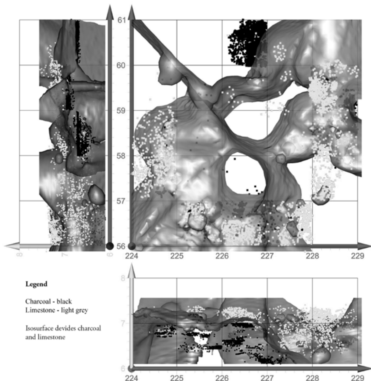
FIG. 6. SPATIAL DISTRIBUTION LIMESTONE AND CHARCOAL FRAGMENTS INSIDE GH 3. ISOSURFACE DIVIDES THEM CLEARLY.
