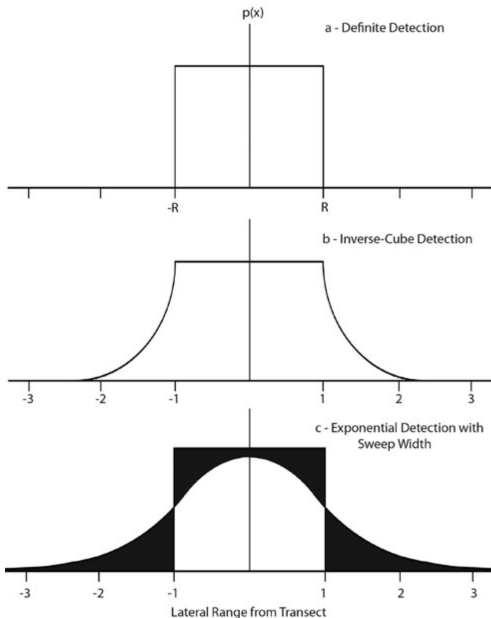
FIG. 4. WITH DEFINITE DETECTION (A), ALL ARTEFACTS WITHIN THE RANGE ( R ) ARE DETECTED, BUT THOSE LYING OUTSIDE THE RANGE ARE NOT DETECTED. INVERSE-CUBE DETECTION (B) ALLOWS FOR A DECREASING PROBABILITY OF DETECTION AS RANGE INCREASES. COMBINING EXPONENTIAL DETECTION WITH SWEEP WIDTH (C) IS AN IMPROVEMENT ON BOTH DETECTION FUNCTIONS (SEE BELOW). THE SHADED AREA ABOVE THE CURVE AND WITHIN R1 REPRESENTS THE ARTEFACTS NOT DETECTED WITHIN THAT RANGE, AND IT IS EQUAL TO THE SHADED AREA BEYOND R1 , WHICH REPRESENTS ARTEFACTS DETECTED BEYOND R1 .
