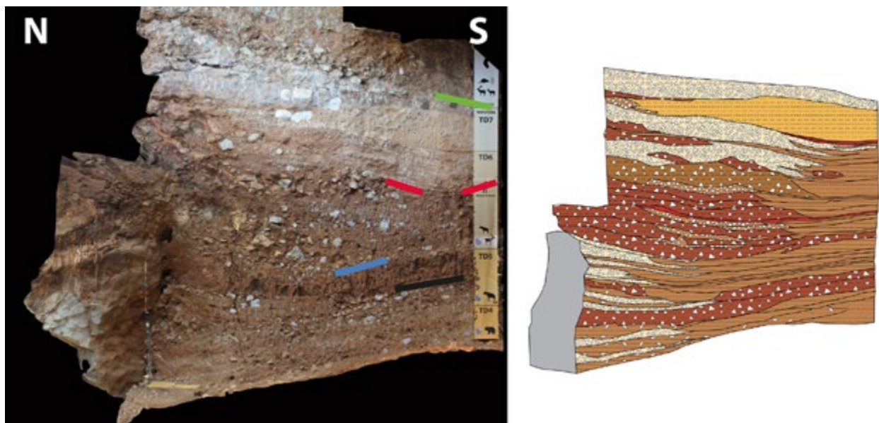
FIG. 6. TD7 TO TD4 SECTION. SILTY LAYERS HAVE POST-DEPOSITIONAL DEFORMATION. TD7 DIP: 11^{\circ} S. TD6.2 DIP: 15^{\circ} . N-S TD6 BASE DIP: 10^{\circ} . N TD5 DIP: 10^{\circ} N.
