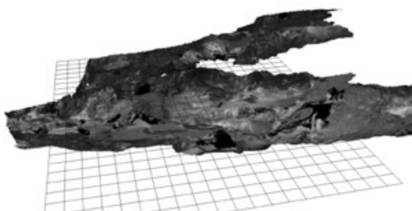
FIG. 13. PROCESSING OF THE 3D SCANNING OF THE CAVE: THE UPPER PART OR THE 'ROOF' HAS BEEN TRIMMED OUT. THIS NEW SURFACE ALLOWS ONE TO PERCEIVE MORE CLEARLY THE INTERNAL AND EXTERNAL PARTS OF THE CAVE LINKED TOGETHER.
