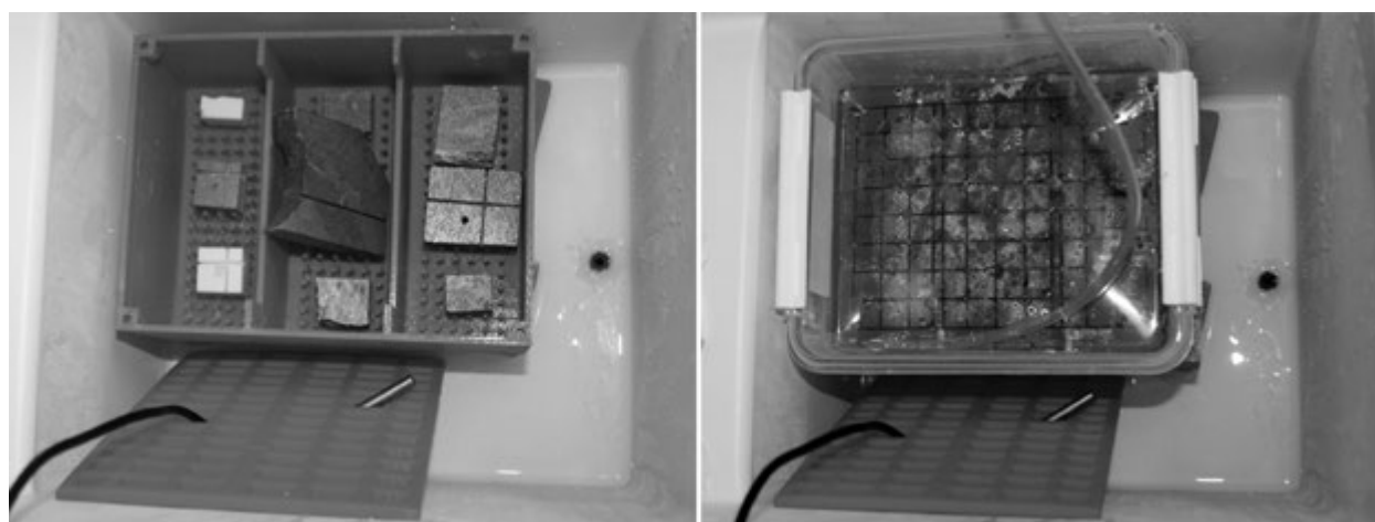
FIG. 10. THE INNER STRUCTURE OF THE FREEZE-THAW CHAMBER. BEFORE A FREEZING CYCLE STARTS, PURIFIED WATER DROPS FOR 30 MINUTES ONTO THE STONES, SIMULATING RAIN.
