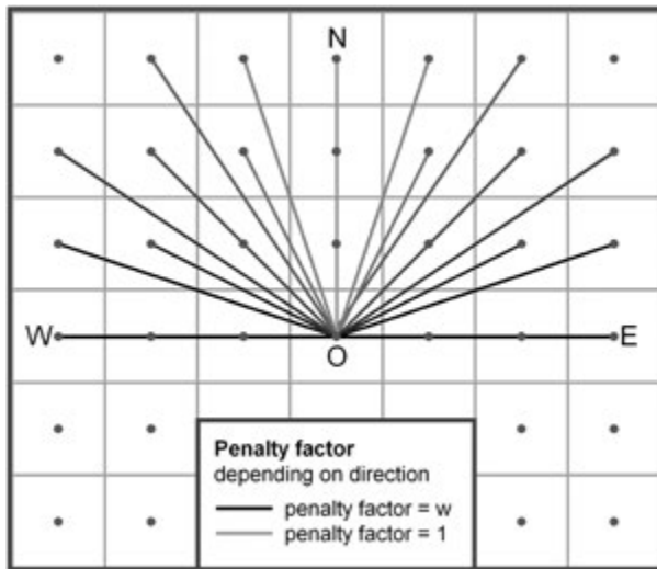
FIG. 3. PENALTY FACTORS FOR CELL O WITH PREFERRED DIRECTION N. MOVEMENTS IN 17 DIRECTIONS ARE SUPPORTED. THE LOWEST PENALTY FACTOR 1 IS ASSIGNED TO THE PREFERRED DIRECTION N, THE HIGHEST PENALTY ( w ) HAS TO BE PAID WHEN MOVING IN A DIRECTION PERPENDICULAR TO THE PREFERRED DIRECTION. A 6 BY 7 CELL GRID IS SHOWN, GRID CELL CENTRES ARE MARKED BY DOTS.
