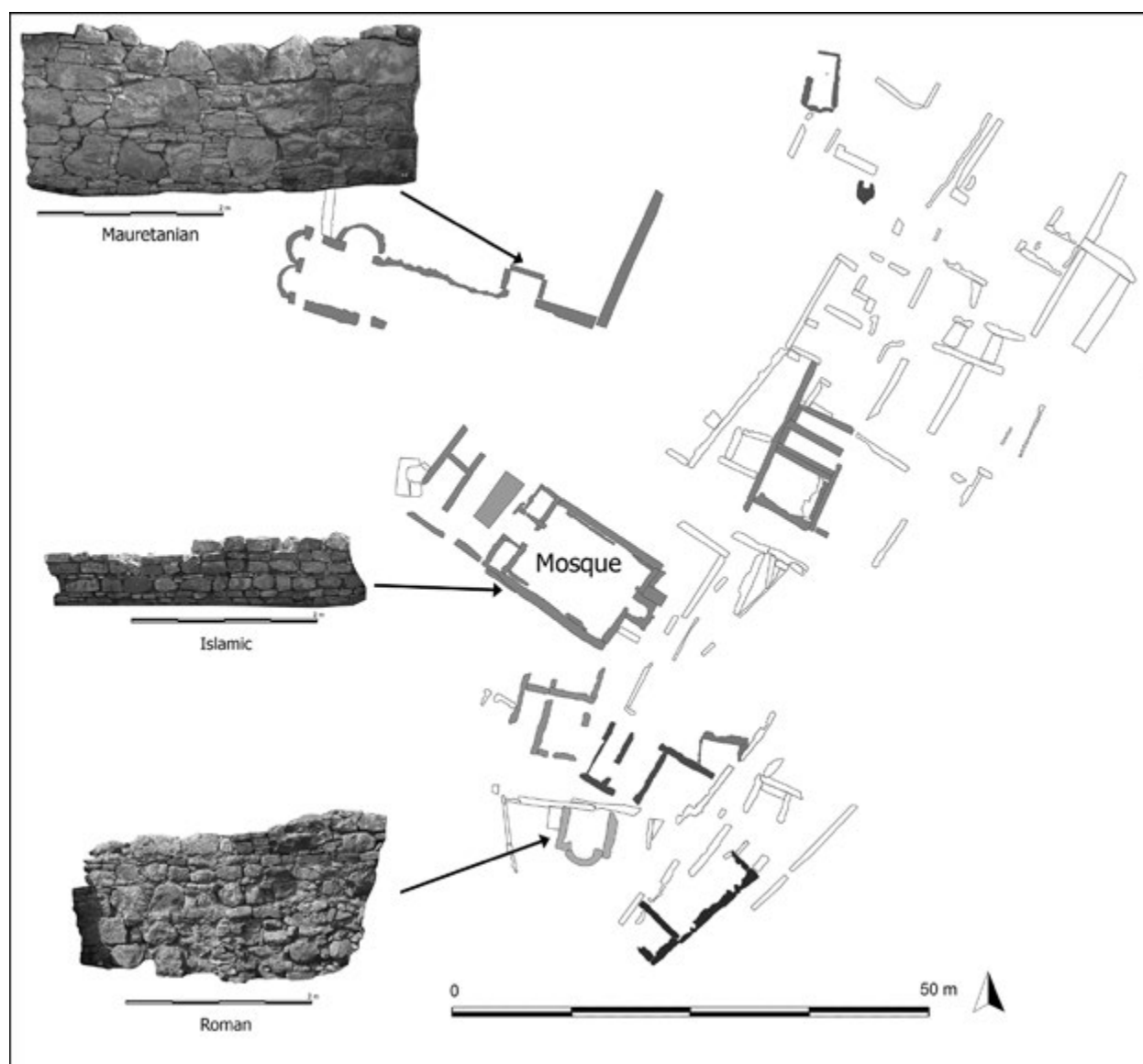
FIG. 7. DETAIL PLAN OF THE MOSQUE AREA, WITH EXAMPLES OF THE BUILDING TECHNIQUES SURVEYED DURING THE FIELD WORK.
