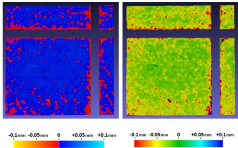
FIG.19. DIFFERENTIAL MAP OF INITIAL TO ERODED MESH FOR THE FRONTAL SURFACE OF THE STONE SLAB ELEFSIS LARGE 3 (EL3): (A) SLABS REGISTERED USING ICP (BLUE INDICATES POSITIVE DISTANCES AND RED INDICATES NEGATIVE DISTANCES); AND (B) SLABS DISPLACED IN Z USING ESTIMATED EROSION VALUE (RED INDICATES MOST ERODED AREAS AND BLUE LEAST ERODED AREAS). COLOURS ARE MAPPED IN THE INTERVAL OF [-0.1MM — +0.1MM]. CONSIDER TWO POINT SETS M = \{M_1, M_2, \dots, M_p\} , THAT REPRESENTS THE INITIAL SURFACE OF A STONE, AND T = \{T_1, T_2, \dots, T_q\} THAT REPRESENTS THE WEATHERED SURFACE OF THE SAME STONE, WHERE M_i, T_j \in \mathbb{R}^3 . THE DISTANCE D_e(M_i) = \min_j (|M_i - T_j|) CAN BE USED AS A LOCAL EROSION MEASURE WHICH EXPRESSES AT EACH VERTEX OF THE INITIAL MODEL M THE DISTANCE OF THE CLOSEST VERTEX OF THE ERODED MODEL T , AND IS A SCALAR MAPPING OF THE EROSION MEASURE AT EACH VERTEX OF THE INITIAL STONE MODEL M , TO WHICH THE ERODED MODEL T IS REGISTERED. |M_i - T_j| IS THE EUCLIDEAN DISTANCE OF A POINT OF M FROM A POINT OF T . FIGURE 19 DEPICTS THE DISTANCE MAPS (I.E. THE D_e(M_i) ) BETWEEN ROUND 01 AND 02 MESHES OF ELEFSIS LARGE 3, AND CONSEQUENTLY THE COMPUTED EROSION MEASURE TEXTURED ON THE INITIAL MESH.
