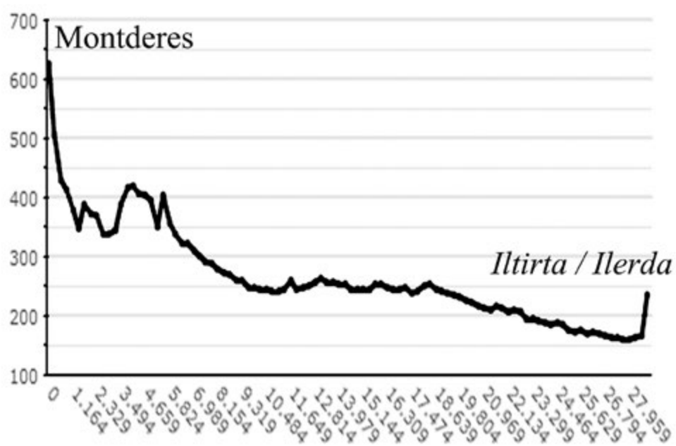
FIG. 12. ALTHIMETRIC PROFILE OF THE MONTERES – ILTIRTA / ILERDA LINE OF SIGHT, PROVIDED BY THE CARTOGRAPHIC AND CATALAN GEOLOGICAL INSTITUTE.
