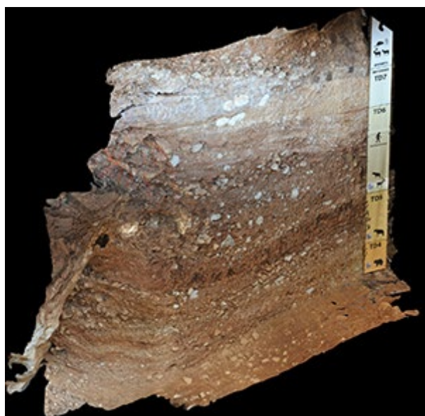
FIG. 3. TD7-TD4 MODEL BY PHOTOGRAMMETRY. 44 IMAGES USED.
