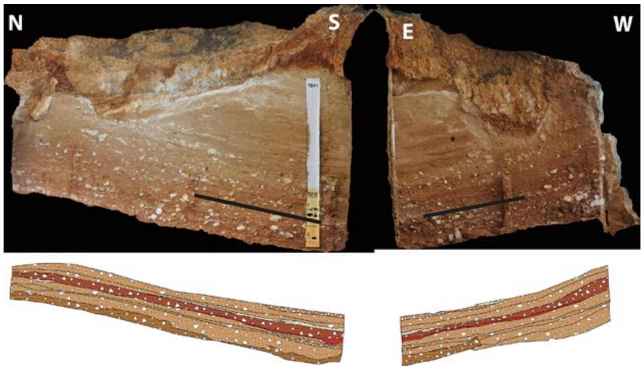
FIG. 5. EAST AND SOUTH SECTION OF TD10. EAST SECTION DIP: 11^{\circ} S. SOUTH SECTION DIP: 11^{\circ} E.
